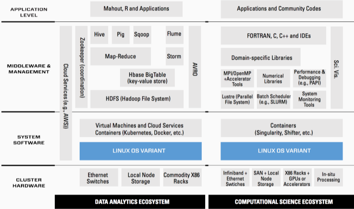
Figure 1: Different software ecosystems for high-end Data Analytics and for traditional Computational Science. [Credit: Reed and Dongarra [66]]
